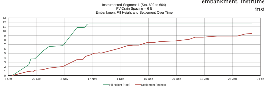
Fill Height and Settlement Over Time - Figure 1
