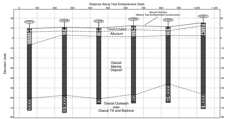
Example of Subsurface Soil Profile
